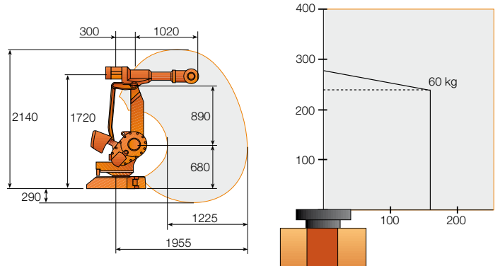
IRB 4400/60
